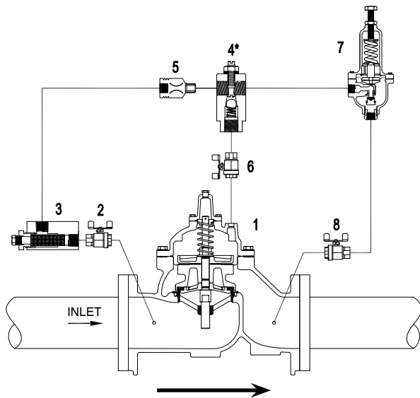
Schematic A-0306C
