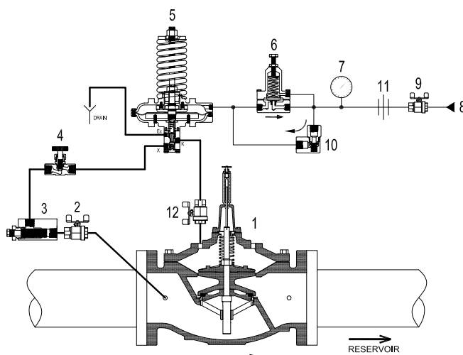
Schematic A-0415C
